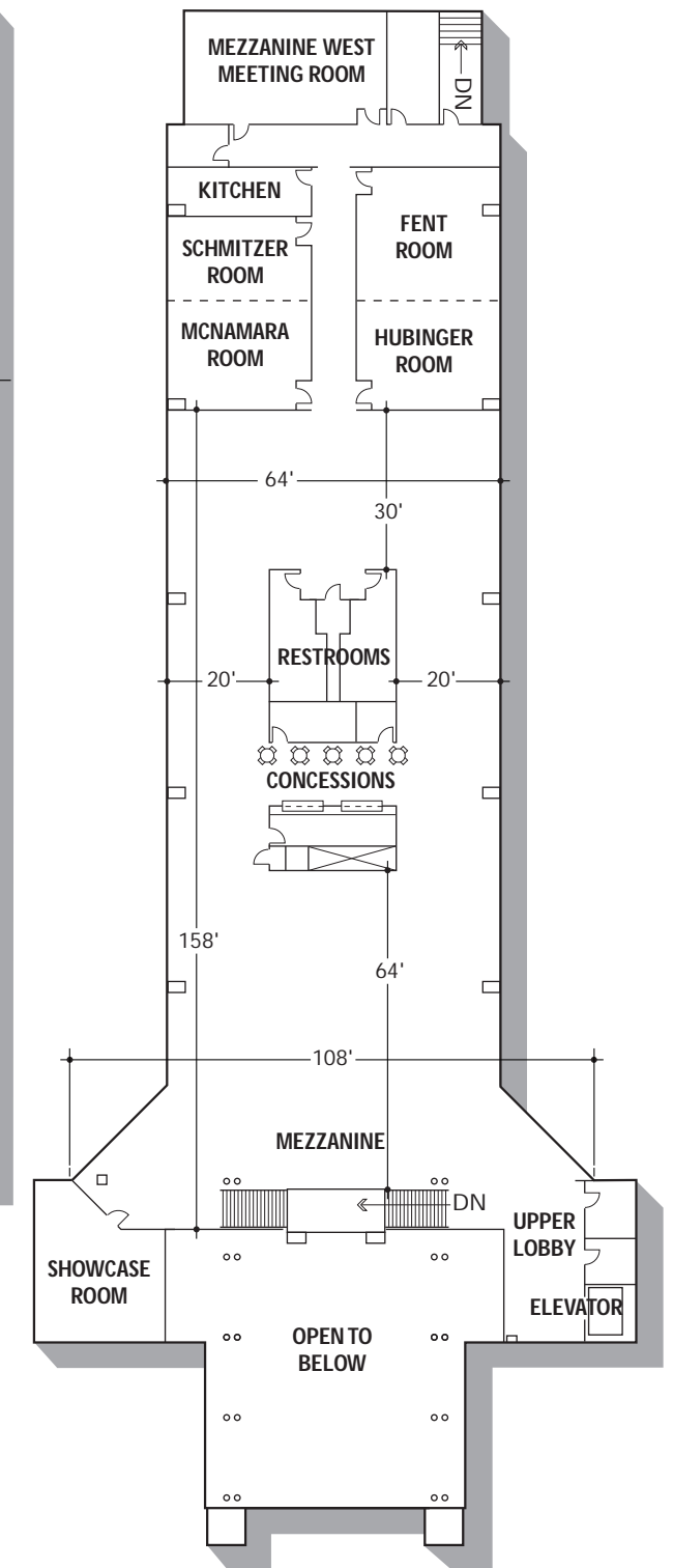
MEZZANINE LEVEL
