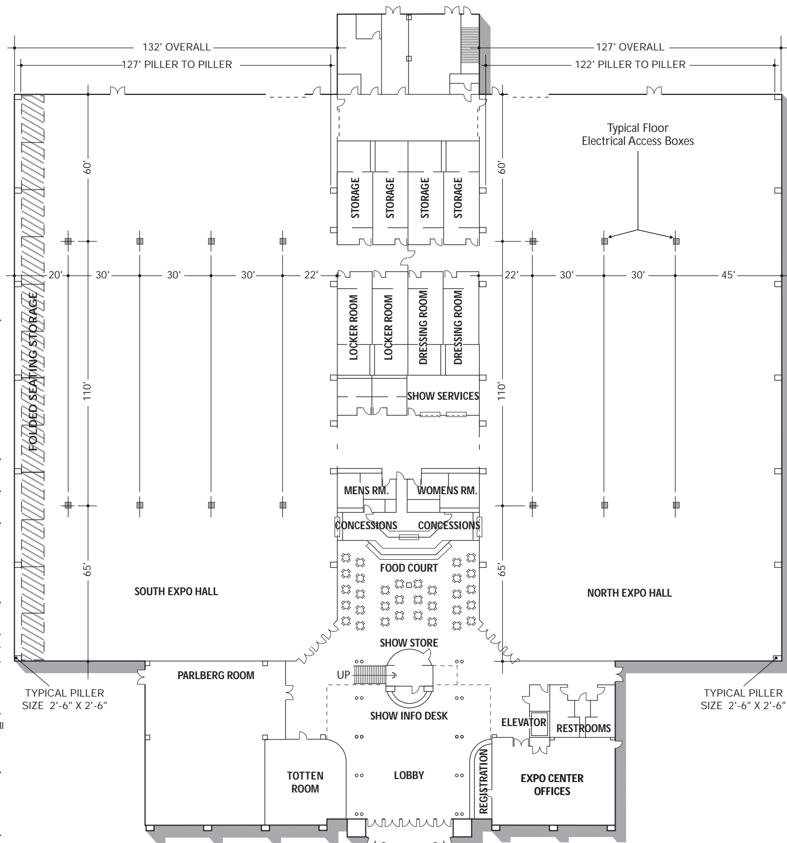
MAIN LEVEL
